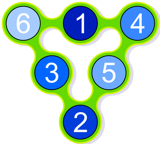
Magic sum 11
