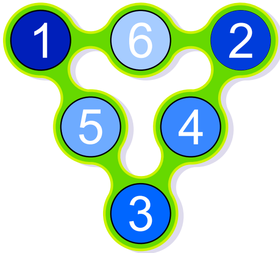
Magic sum 9
