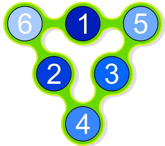
Magic sum 12
