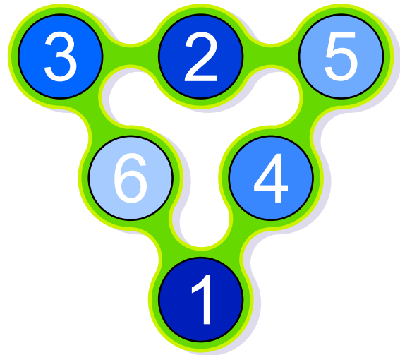
Magic sum 10
